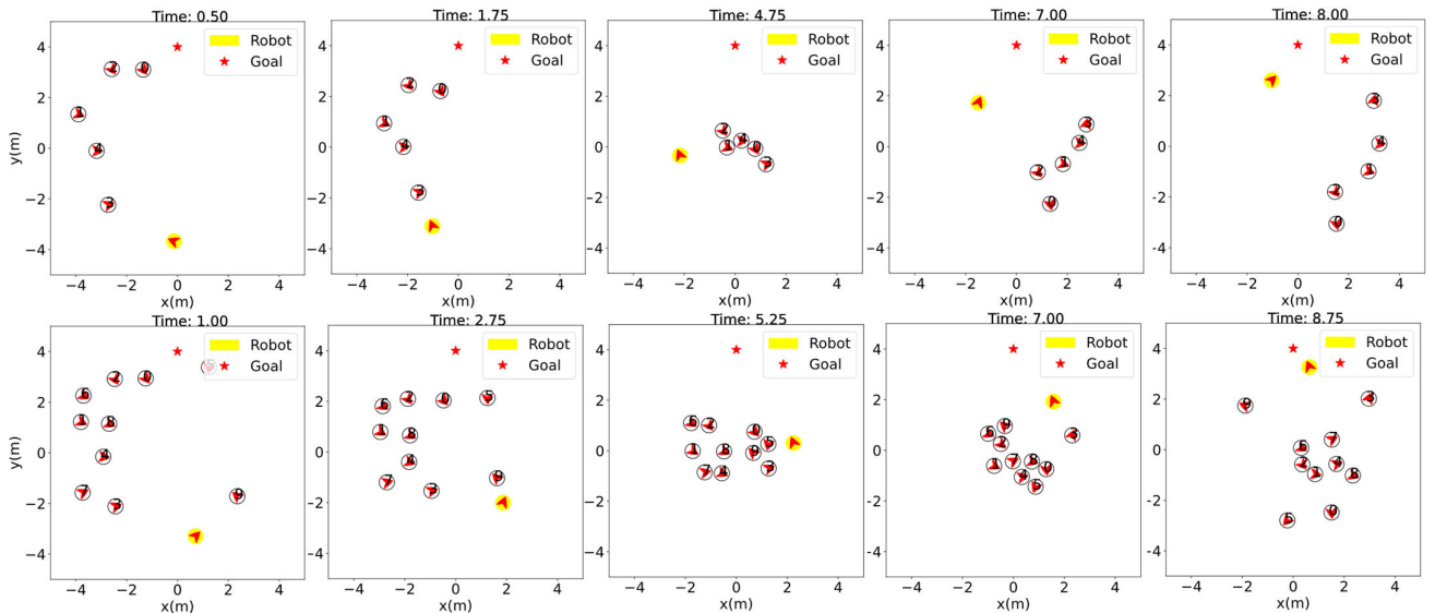
Fig. 9. Motion planning process (ALN-DSAC) in cases with five and ten obstacles.
