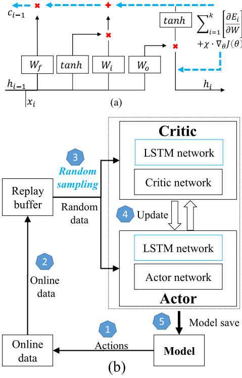
Fig. 4. Architecture of LSTM-DSAC. (a) LSTM backpropagation. (b) LSTM-DSAC architecture.
