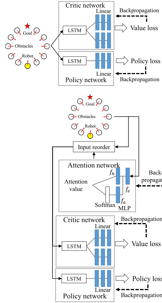
Fig. 7. Network frameworks. The first framework is for LSTM-DSAC, while the second is for AL-DSAC and ALN-DSAC.
