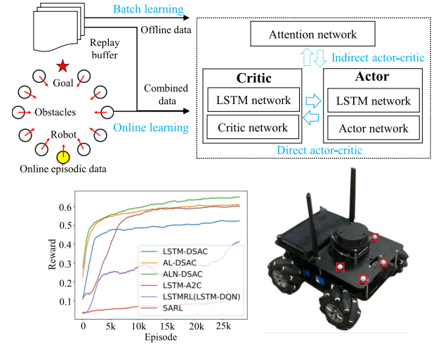
Fig. 1. Workflow of ALN-DSAC. LSTM/AL-DSAC denotes the DSAC with LSTM or attention-based LSTM encoders.
