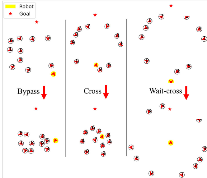
Fig. 10. Learned motion planning strategy.
