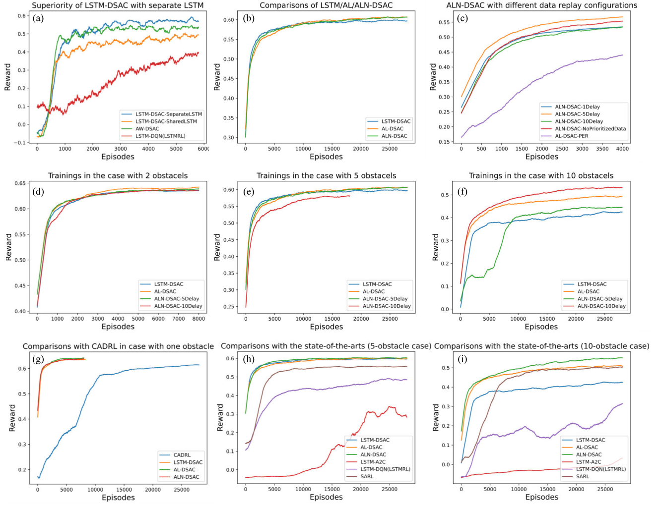
Fig. 8. Training results. In (c), ALN-DSAC-1/5/10Delay denotes the novel data replay with one/five/ten delayed experiences. ALN-DSAC-NoPrioritizedData denotes that the prioritized sampling method-1/2 is replaced by random sampling in the novel data replay. AL-DSAC-PER denotes that AL-DSAC uses classical PER. In (g), CADRL does not support multiobstacle training. Its networks are trained in one-obstacle case, and trained models can be applied to multiobstacle motion planning. Hence, the training of CADRL is presented in independent figure.
